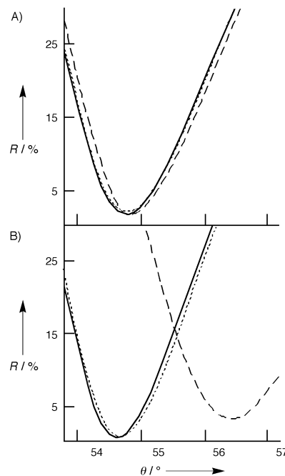
Figure 16. In situ SPR curves of: A) An evaporated gold film, modified with anti-IgG- \gamma (—) and sequentially exposed to IgG ( 0.045 \text{ mg mL}^{-1} ; ....) then anti-IgG- F_c ( 8.5 \text{ mg mL}^{-1} ; ---); B) The same experiment, except that the final anti-IgG- F_c was conjugated with 10 nm gold nanoparticles. R = resonance enhancement. Reproduced from ref. [215] with permission.
